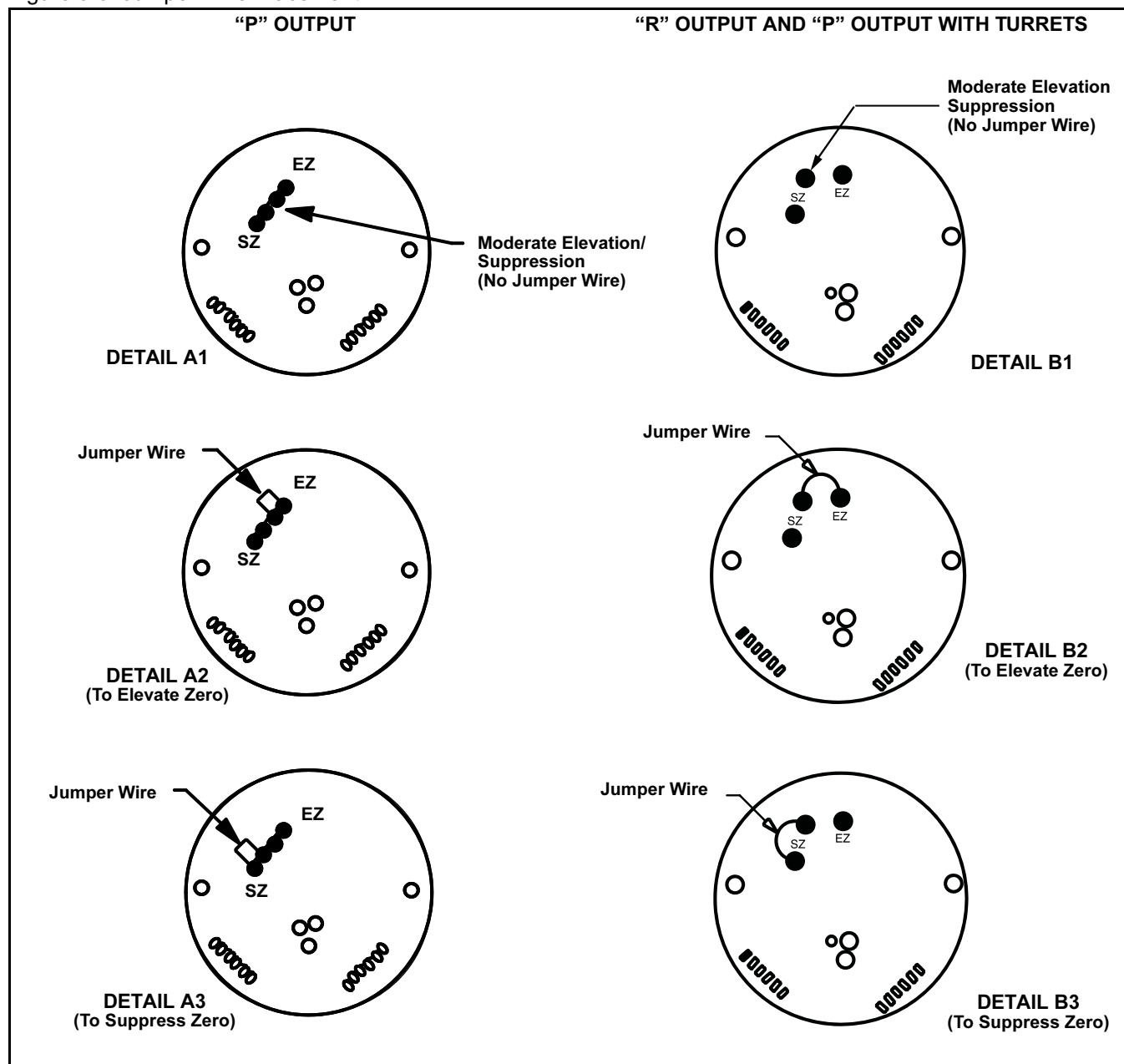
Figure 3-3. Jumper Wire Placement.
