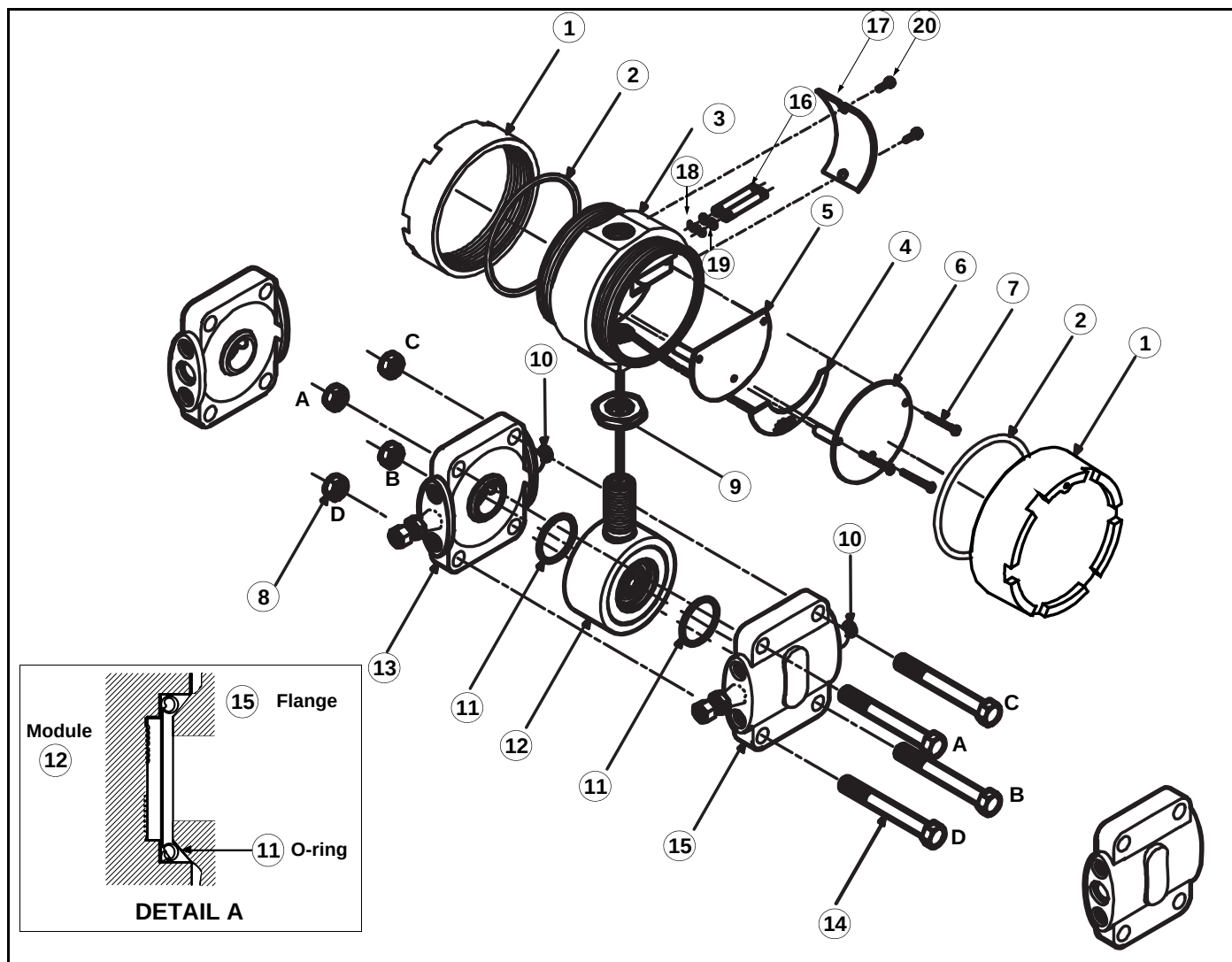
Figure 5-2. Typical Rosemount 1153 Series D Exploded View.
